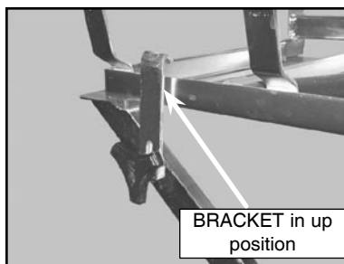
(E) Seat Front Side of saw onto stand and make sure that the BRACKET is in the up position
