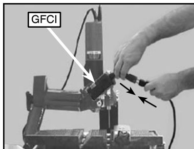
(B) Plug MK-770 EXP into the GFCI
