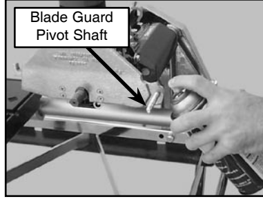
(E) Remove the Blade Guard then clean and Lubricate the Blade Guard Pivot Shaft
