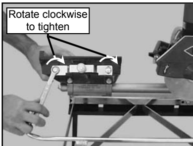
(P) Verify the Cutting Table Roller Wheel Assembly is tight
