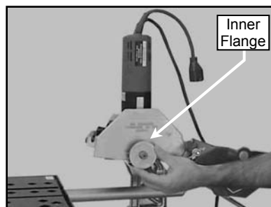
(B) Remove the Inner Flange
