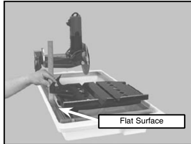
(B) Place Square on guide bar side of cutting table
