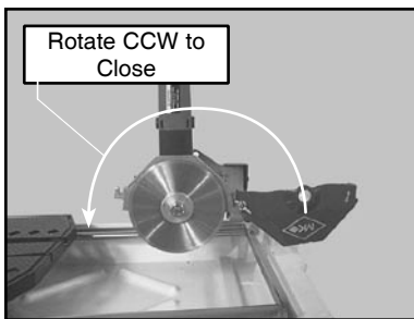
(G) Close the Outer Blade
