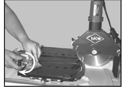
(C) Position the Dual 45° Flat Angle Guide and tighten the retaining knob
