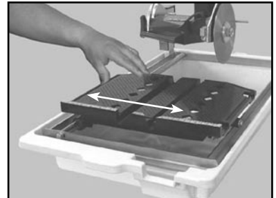
(F) Move Guide Bar and table until Square rests evenly across Blade
