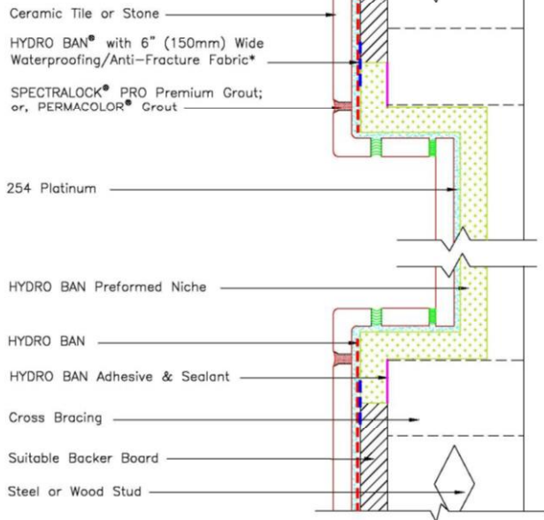
Drawing No. ES-W244N Single Panel
