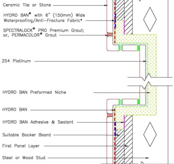
Drawing No. ES-W244N Double Panel
